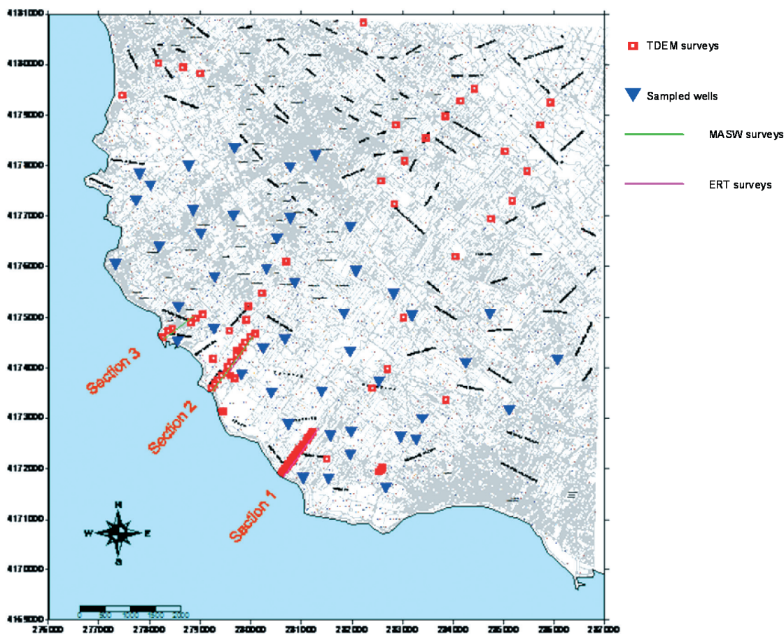
Fig. 2 - Geophysical and hydrogeochemical monitoring network.
