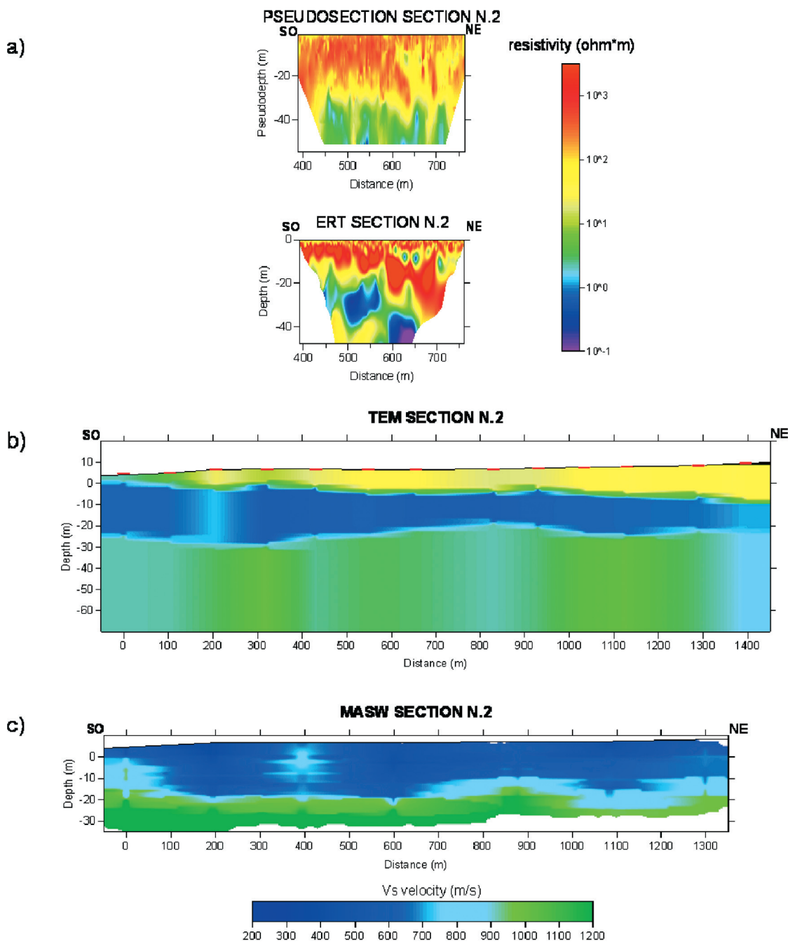
Fig. 5 - 2D interpretation of ERT survey (a), TEM soundings (b) and MASW measurements (c) relative to Section n°2.
